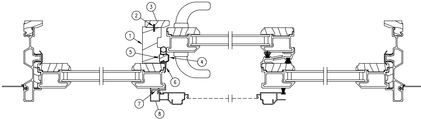
3 Panel Jamb Detail - OXO R
