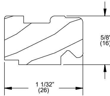
Head Jamb Liner, W7624 Replace with W8565
