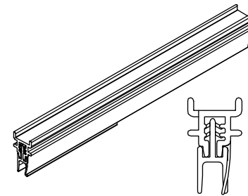
Screen Roller Guide Assembly Replace with V552
