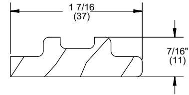
Stationary Panel Spacer, W7626 Replace with W8581
