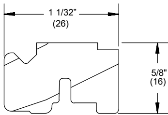
Head Jamb Liner, W7709 Replace with W8565
