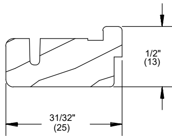
Operator Panel Guide W7625 Replace with W7710
