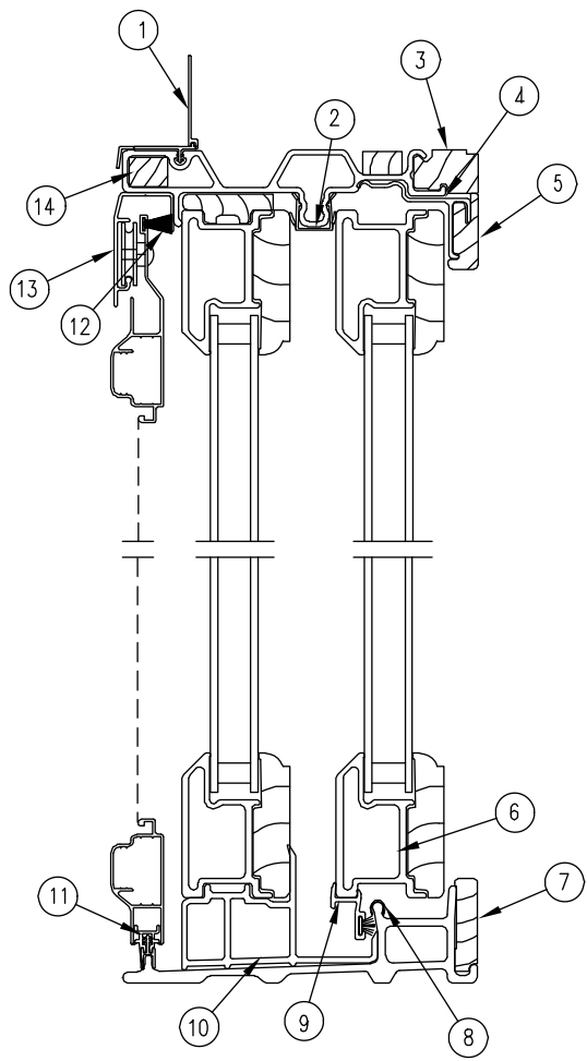
Head Jamb and Sill Detail
