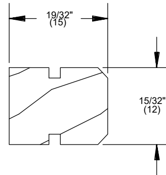
Astragal Parting Stop, W7716 Replace with the Astragal Assembly
