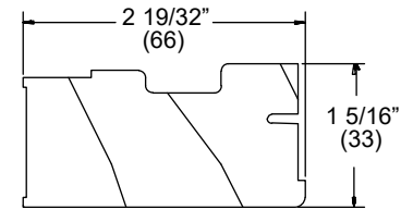
Astragal, W7717 Replace with the Astragal Assembly
