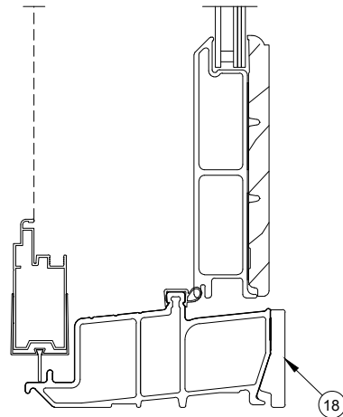
Sill Detail, HP/IZ3
