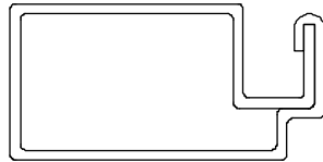
Screen Surround, Aluminum Profile, A135
