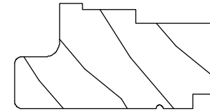
Jamb Liner with Interior Stop, W10917 Max length: 76" (1930)
