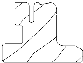
Interior Astragal, W12643 OXXO Max length: 96" (2438)
