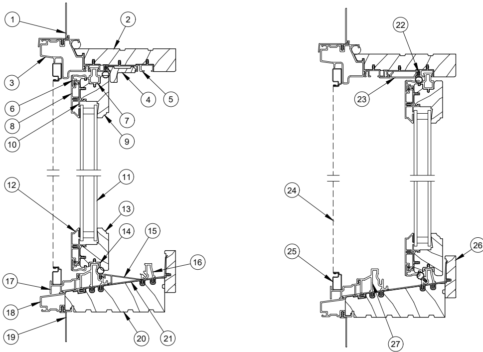
Head Jamb and Sill Detail
