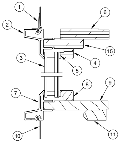
Head Jamb & Sill Detail
