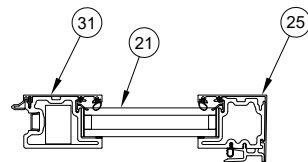
15/16 Bi-parting Panel
