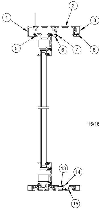
Stationary/Pocket Panel Head Jamb and Sill
