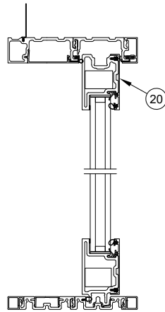
Primary/Inactive Panel Head Jamb and Sill
