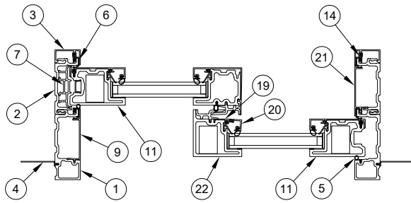
Stacked Uni-directional Jamb Detail
