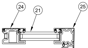
15/16 Uni-directional Panel
