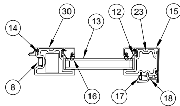
15/16 Bi-parting Panel
