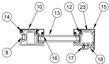
15/16 Uni-directional Panel
