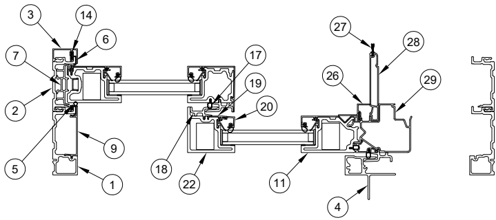
Pocket Uni-directional Jamb Detail
