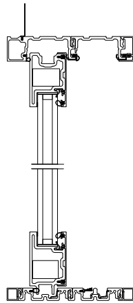
Stationary/Pocket Panel Head Jamb and Sill
