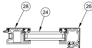
1 5/16" Bi-parting Panel
