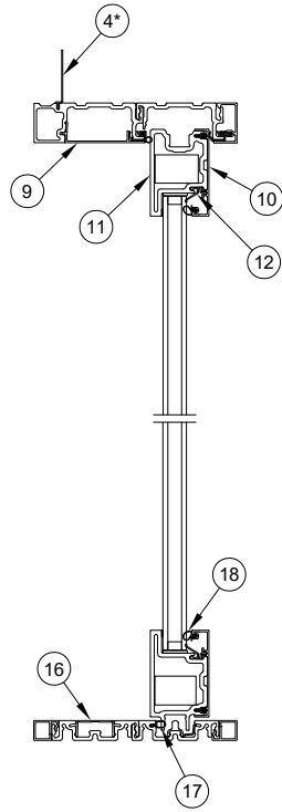
Primary/Inactive Panel Head Jamb and Sill
