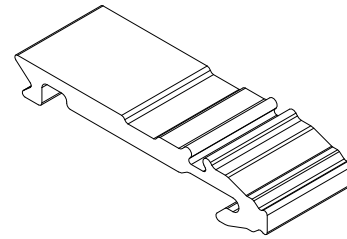
MRF, 1/2" Sill/LH Jamb, F4033 Casement, Awning, Direct Glaze Rectangle
