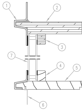
Head Jamb and Sill Detail
