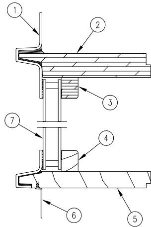
Head Jamb and Sill Detail
