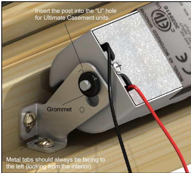
Figure 1: Bracket orientation
