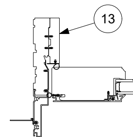
6 9/16" Jambs - 2 1/4" Panel
